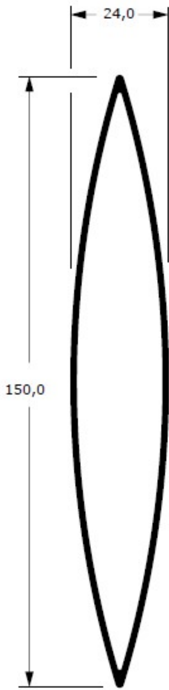
DC-004 1,300 kg/m
