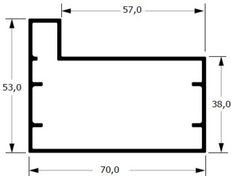
PC-010 1,119 kg/m
