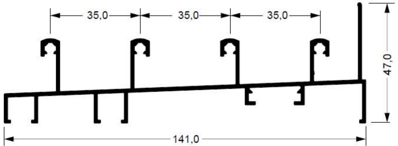
SU-122 1,509 kg/m
