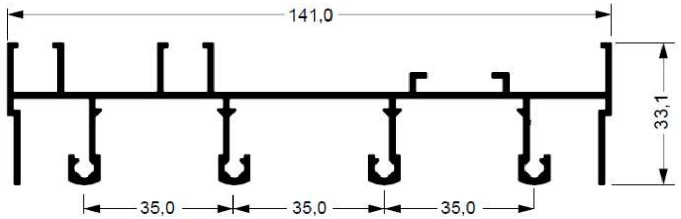
SU-121 1,585 kg/m
